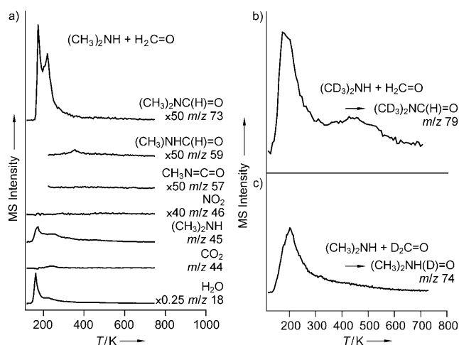
Figure 1. Reaction of dimethylamine and formaldehyde on O/Au(111) yields N,N -dimethylformamide in temperature-programmed reaction spectra obtained after introducing: a) [\text{D}_0] dimethylamine (9 L) and b) [\text{D}_6] dimethylamine ( (\text{CD}_3)_2\text{NH} ) (9 L) both followed by [\text{D}_0] formaldehyde (27 L) on O/Au(111) ( \theta_{\text{O}} = 0.15 ML) at 120 K. In c) [\text{D}_0] dimethylamine (9 L) and [\text{D}_2] formaldehyde (27 L) were sequentially dosed onto O/Au(111) ( \theta_{\text{O}} = 0.15 ML) at 120 K. The contributions from fragmentation of dimethylamine and N,N -dimethylformamide to the m/z 44 and m/z 46 signals were subtracted for clarity in (a). No reaction is detected on clean Au(111). The heating rate was 4 \text{ K s}^{-1} .
