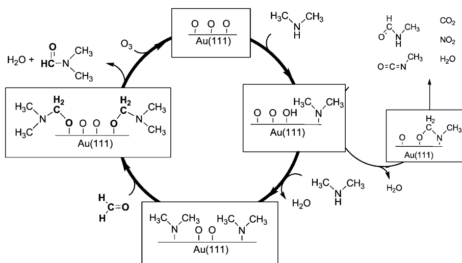
Scheme 1. Proposed mechanisms for the coupling of dimethylamine with formaldehyde and the secondary oxidation of dimethylamine promoted on O/Au(111).
