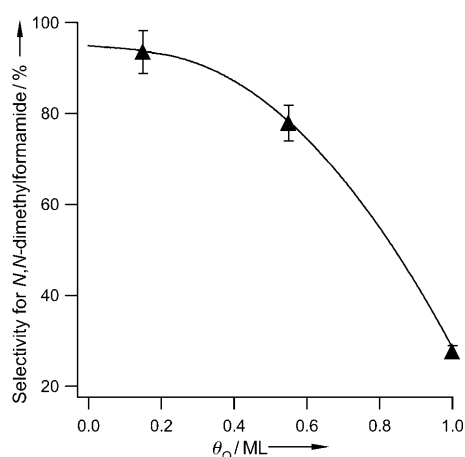
Figure 2. Selectivity for production of N,N -dimethylformamide (the ratio of m/z 73 signal to the sum of m/z 44 and m/z 73 signals, corrected for fragmentation) vs. initial oxygen coverage.
