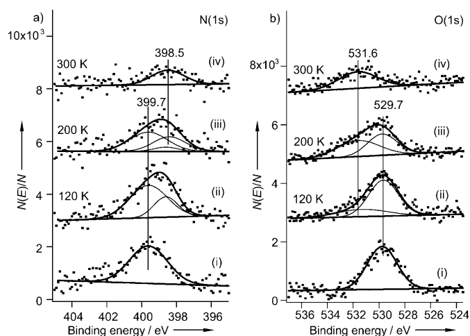
Figure 3. X-ray photoelectron spectra. a) N(1s) region following: i) condensation of dimethylamine multilayers on Au(111) at 120 K, ii) adsorption of dimethylamine on O/Au(111) ( \theta_{\text{O}} = 0.15 ML) at 120 K and subsequently heated to iii) 200 K and iv) 300 K. b) O(1s) region for: i) as-prepared O/Au(111) ( \theta_{\text{O}} = 0.15 ML) and ii–iv) after the same treatment as in (a), plots ii–iv. All spectra were obtained after cooling to 120 K.
